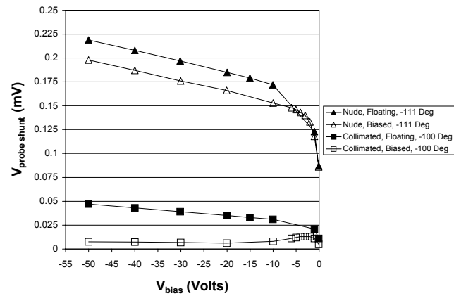
Figure 11 – Effect of varying the probe bias at several angular positions. Cases when the guard ring/collimator are biased and floating are shown. (300 V, 4.5 A thruster operation)
