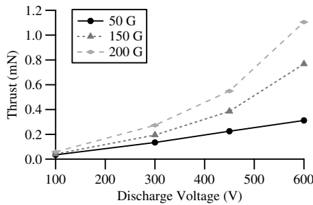
Fig. 24 Estimated thrust as function of discharge voltage and magnetic field; 429 W RF power, 1.5 mg/s argon, 35 V screen grid bias, 150 V accel grid bias, 1.6 \times 10^{-5} torr Ar chamber pressure.
