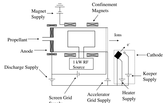
Fig. 2 GHIT configuration.
