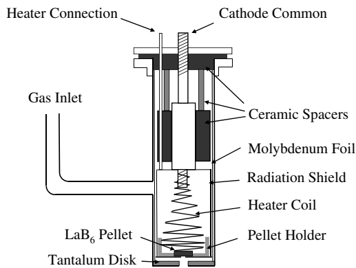
Fig. 7 Cathode schematic.
