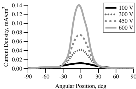
Fig. 21 Plume current density as function of discharge voltage 50 cm from grids; 429 W RF power, 150 G magnetic field, 1.5 mg/s argon, 35 V screen grid bias, 150 V accel grid bias, 1.6 \times 10^{-5} torr Ar chamber pressure.
