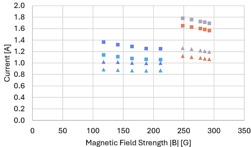
Fig. 12 Discharge and beam current vs B field strength
