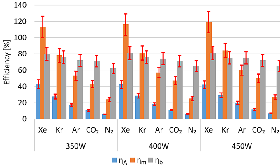
Fig. 8 Thruster efficiencies for fixed voltage (250V) and fixed power
