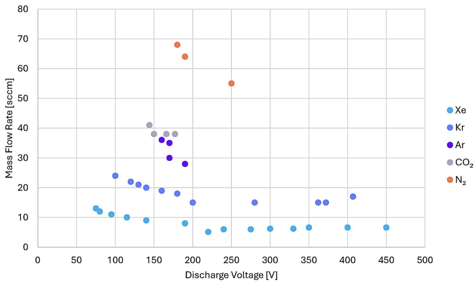
Fig. 6 Operational envelope. Minima points that allow stable thruster operation ( >300 s) without thruster spontaneous shutdown
