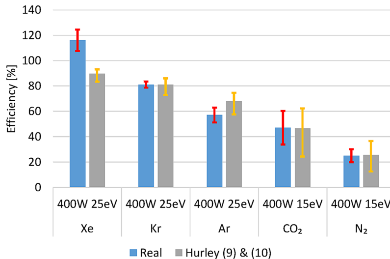
Fig. 9 Experimental vs Hurley's model \eta_m
