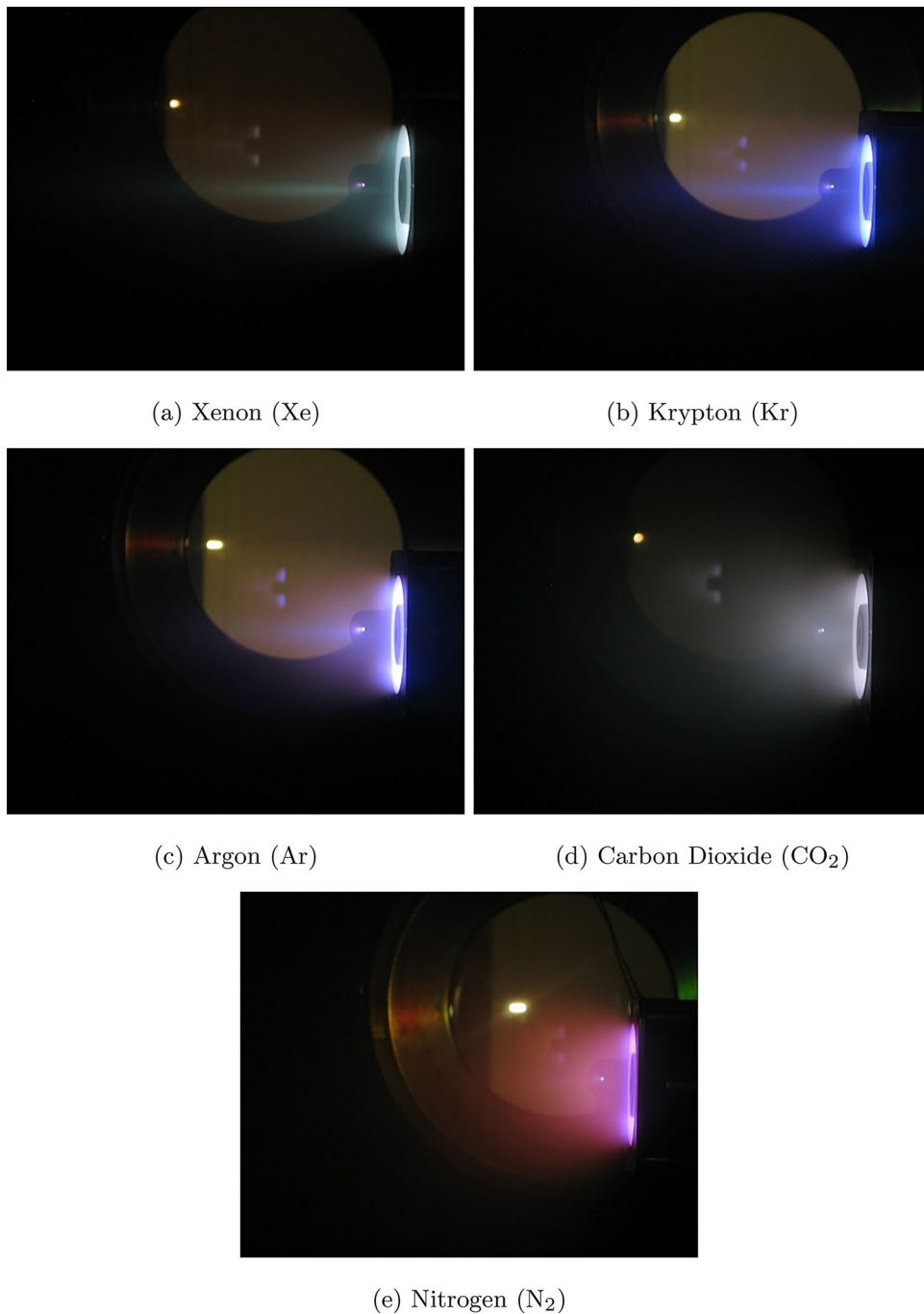
Fig. 5 Thruster operating on five gases: xenon, krypton, argon, CO 2 , and N 2
