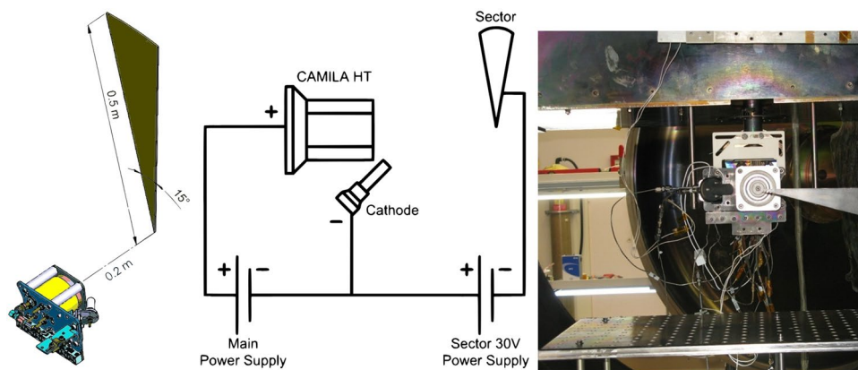
Fig. 4 Diagram and picture of the angular faraday probe [21]
