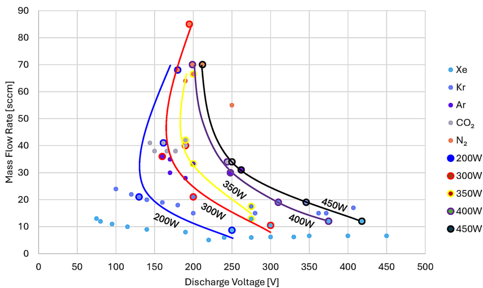
Fig. 7 Operational envelope with non-unique equi-power lines. the bullet color represents the gas type, while the bullet outline color (for relevant points) represents the power level
