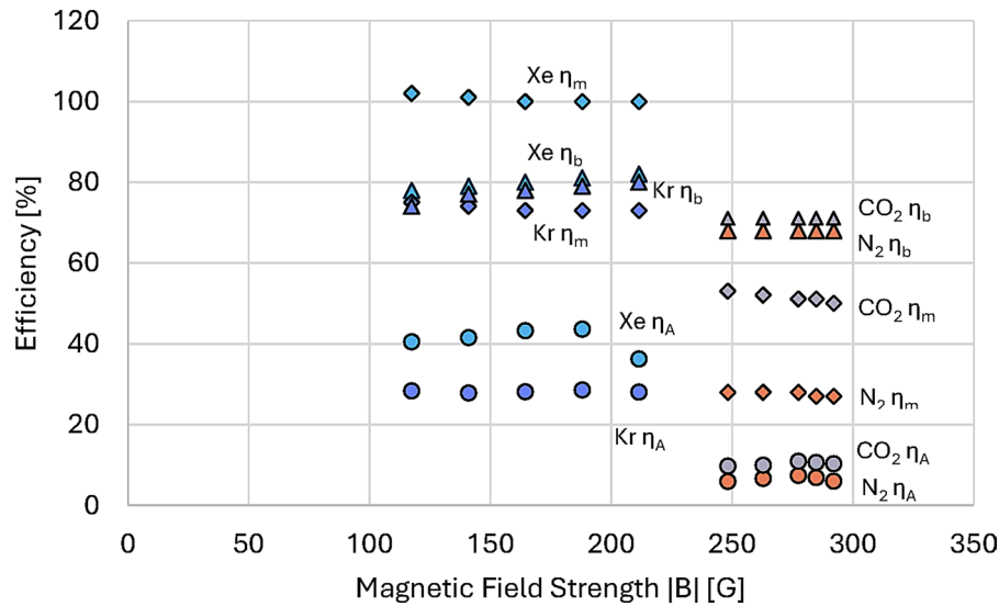
Fig. 10 Internal efficiencies as a function of B field strength
