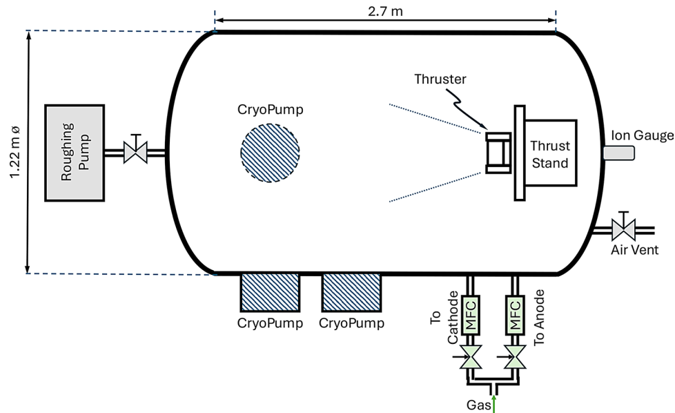
Fig. 3 Schematic of the Asher Space Research Institute (ASRI) electric propulsion laboratory experimental facility. (not to scale)
