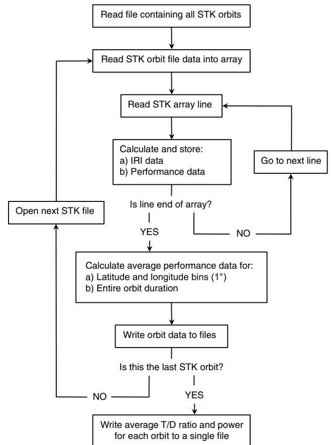
Fig. 2 AEPMPT path including nested loops, IRI integration, and data output.
