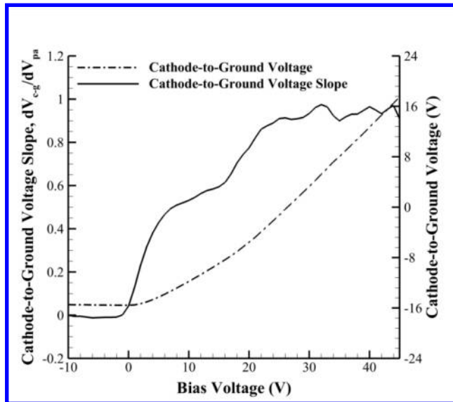
Figure 7. Measured T-140 HET cathode-to-ground voltage and its derivative with respect to axial plate bias voltage as a function of bias voltage.
