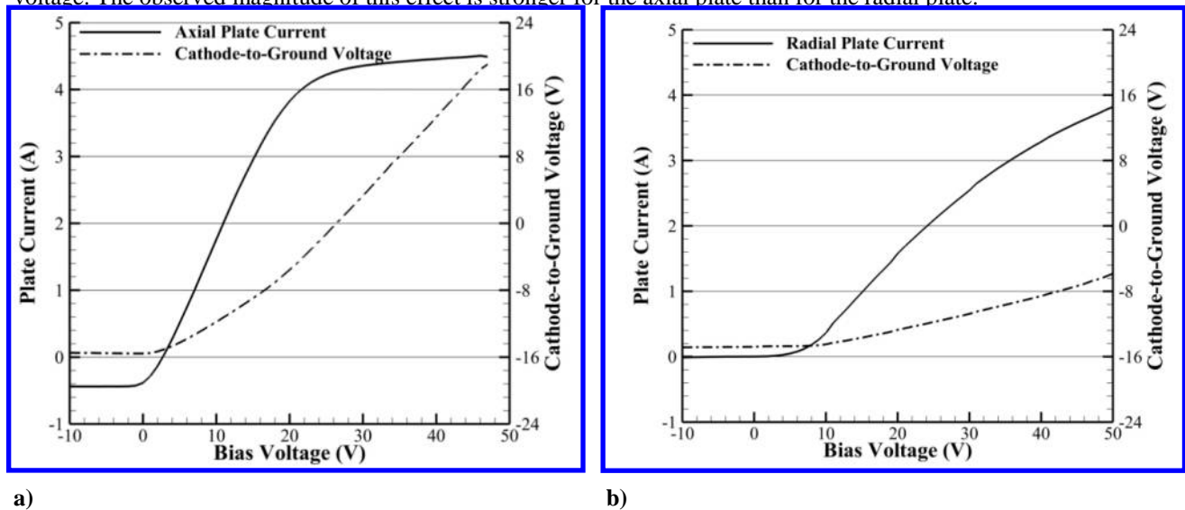
Figure 3. T-140 HET cathode-to-ground voltage and plate current of the: a) axial and b) radial plates measured during IV sweeps.
