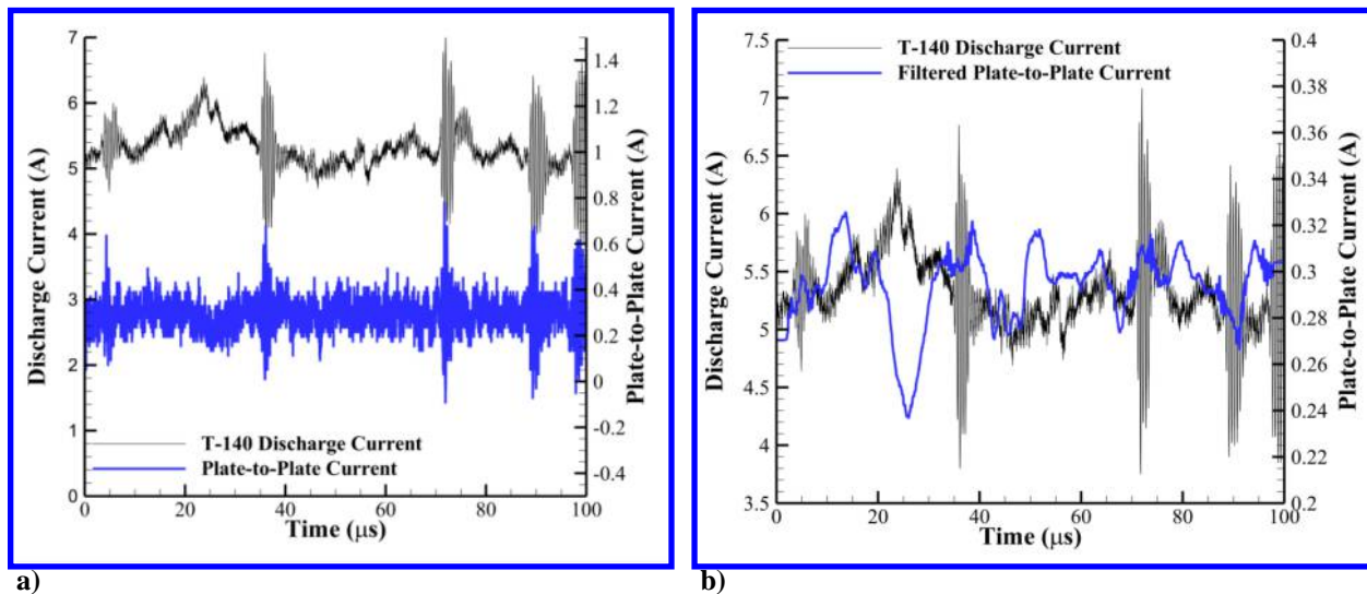
Figure 6. T-140 HET discharge current oscillations and a) unfiltered and b) moving average filtered plate-to-plate current for the connected plate configuration.
