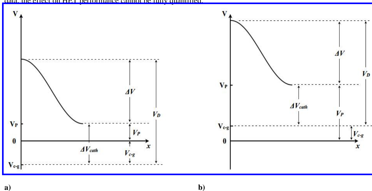
Figure 8. T-140 HET potential distribution for the a) grounded and b) positively-biased plates.
