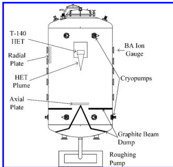
Figure 1. Schematic of VTF-2 (not to scale).
