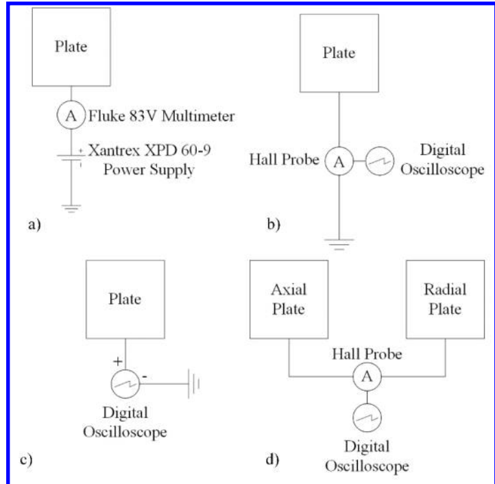
Figure 2. Plate circuit configurations: a) IV-swept, b) grounded, c) floating, and d) connected.
