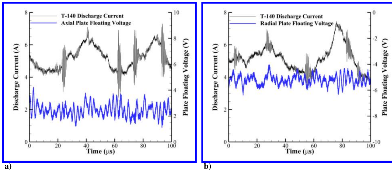
Figure 5. T-140 HET discharge current oscillations and plate floating voltages measured for the floating configuration of the: a) axial and b) radial plates.
