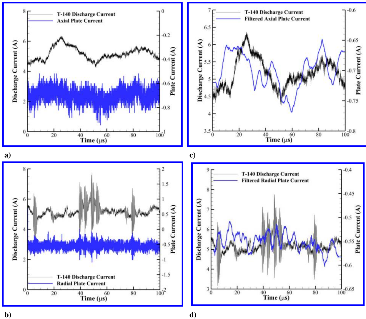
Figure 4. T-140 HET discharge current oscillations and plate current collected for the grounded-plate configuration: a) unfiltered axial plate current, b) unfiltered radial plate current, c) moving-average filtered axial plate current, and d) moving-average filtered radial plate current.
