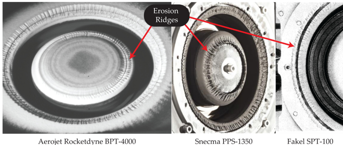
Figure 6. Erosion ridges in the Aerojet Rocketdyne BPT-4000, Snecma PPS-1350, and Fakel SPT-100 walls. Images reprinted with permission from [18], Aerojet Rocketdyne, 2010; with permission from [66], Snecma, 2019; and with permission from [15], American Institute of Aeronautics and Astronautics, 1995.
