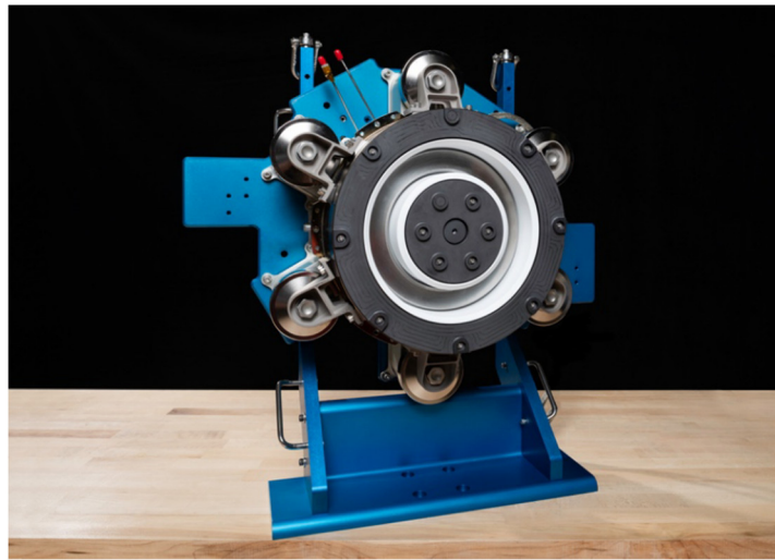
Figure 8. Magnetically-shielded Advanced Electric Propulsion System (AEPS) Engineering Test Unit 1. Image reprinted with permission from [11], NASA, 2019.
