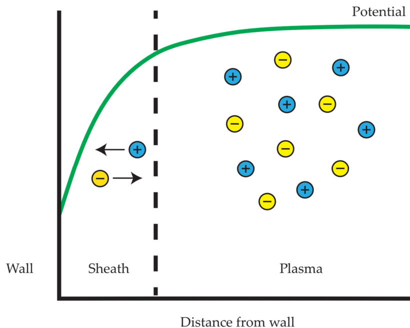
Figure 3. Simplified illustration of the potential drop in the wall sheath [24]. The potential gradient in the sheath repels electrons (yellow) away from the wall and accelerates ions (blue) toward the wall.
