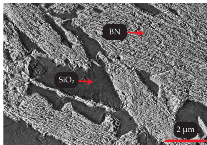
Figure 4. Scanning electron microscopy (SEM) image of grade M26 BN-SiO 2 . The dark regions are amorphous silica (SiO 2 ) and the light regions are orthotropic boron nitride (BN).
