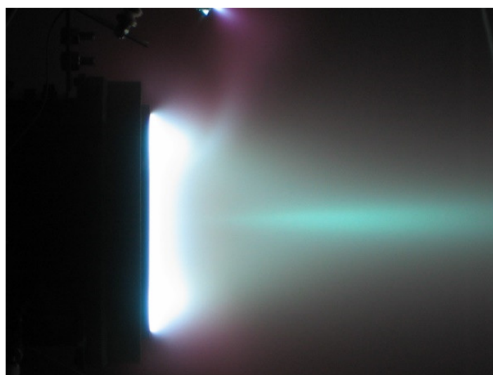
Figure 1. Pratt & Whitney T-140 Hall thruster operating with xenon propellant.
