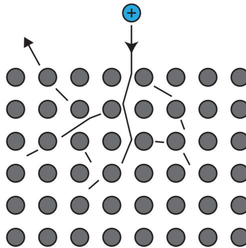
Figure 5. Sputtering mechanism according to the transport model [33]. An incident ion (blue) transfers energy to atoms (grey) and the resulting collision cascade propels an atom away from the surface.
