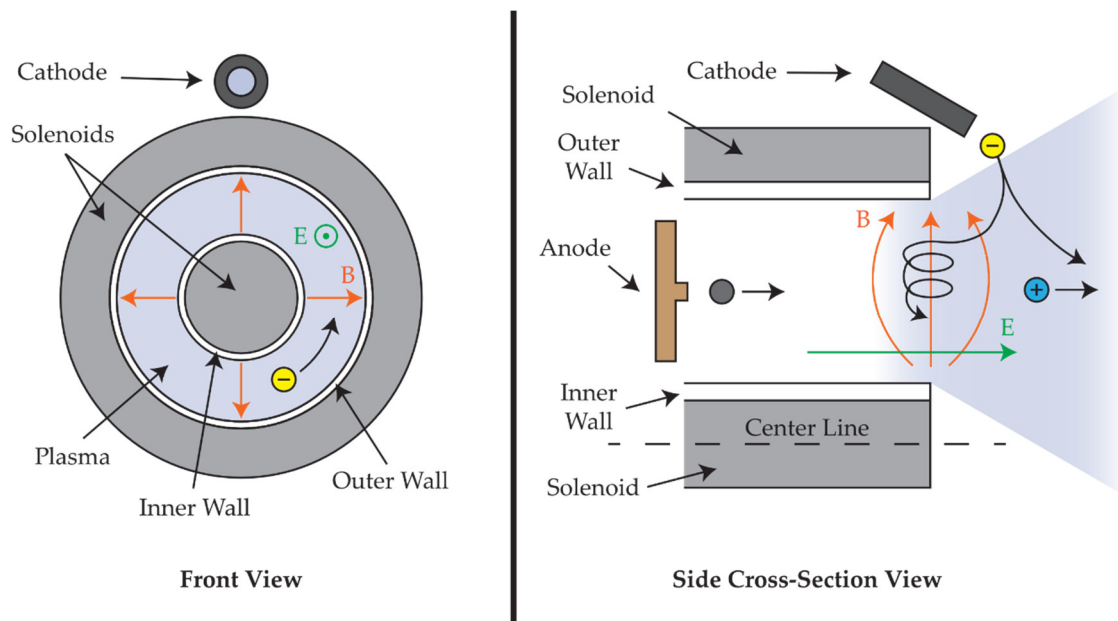
Figure 2. Front and side cross-section schematics of a Hall thruster [3,7]. Electrons (yellow) trapped in a Hall drift by crossed electric (green) and magnetic (orange) fields ionize neutral (grey) propellant. The resulting ions (blue) are accelerated into the thruster plume by the electric field.
