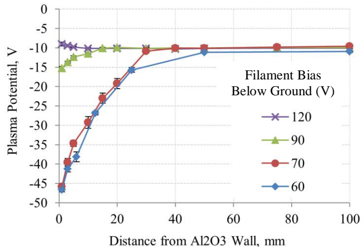
Figure 3. Measurements of sheath potential profile over alumina surface. For all cases, neutral pressure is 7.5 \times 10^{-5} Torr-Ar with 10.0 mA discharge current.
