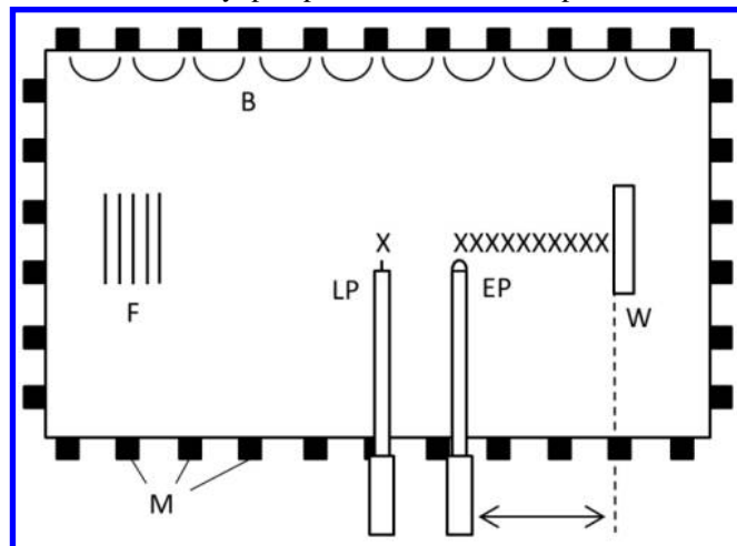
Figure 1. Schematic of experiment layout. F = filaments, M = magnets, B = nominal magnetic field, LP = Langmuir probe, EP = emissive probe, W = wall material sample, X = nominal data measurement location. Emissive probe orientation rotated 90° in figure to show hairpin tip geometry. Figure not to scale.
