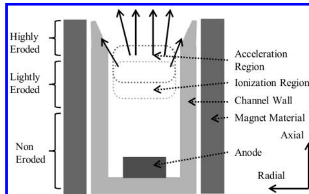
Figure 1. Erosion process in HET discharge channel
